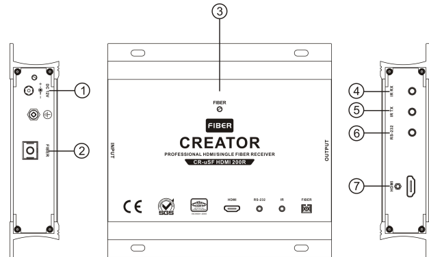
CR-uSF HDMI 200R rear panel :
