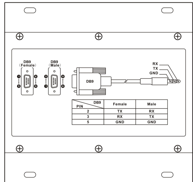
CR-uSF HDMI 200R rear panel :
