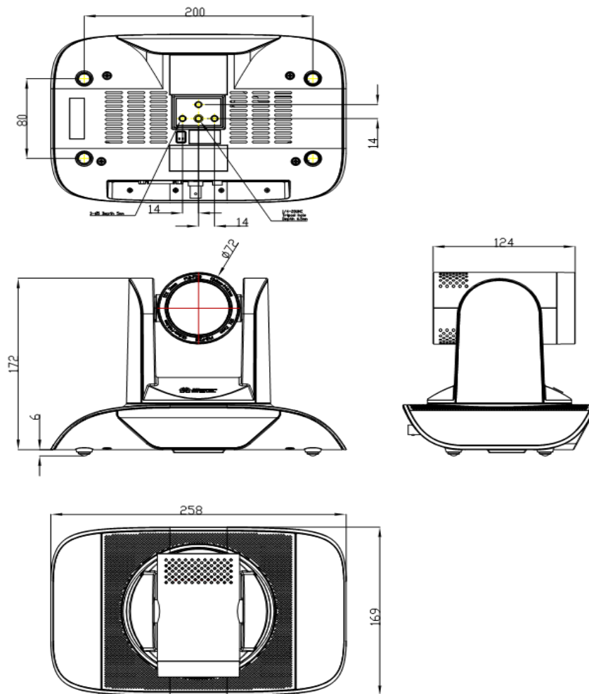
Figure 2.2 Camera dimension
