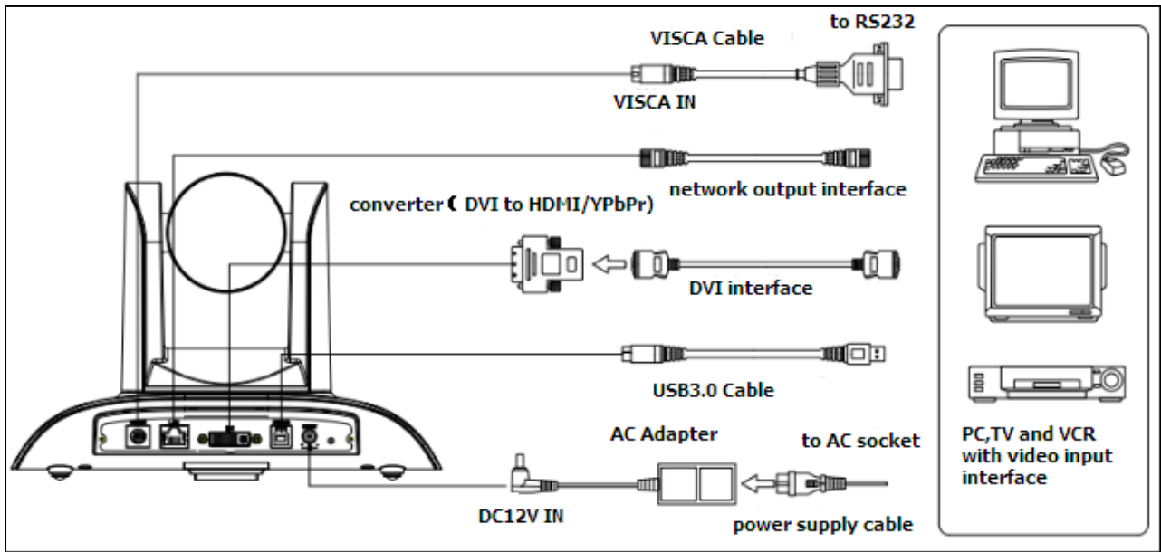
Figure 2.4 U3 model external interface diagram
