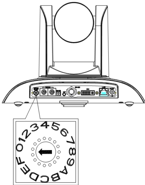
Figure 2.6 Rotary Dial diagram
